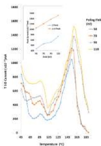
Figure 2 : TSDC thermograms for PVP samples poled at 70 oC with different poling fields (i.e. 50, 70, 90 and 110 kV/cm).
