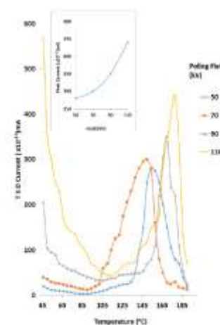
Figure 3 : TSDC thermograms for 95:05 polyblend samples poled at 70 oC with different poling fields (i.e. 50, 70, 90 and 110 kV/cm).
