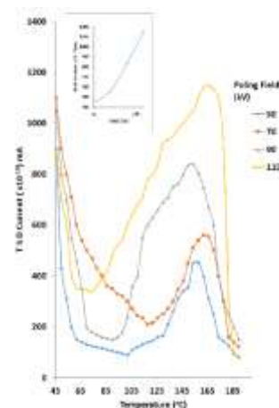
Figure 6 : TSDC thermograms for 80:20 polyblend samples poled at 70 oC with different poling fields (i.e. 50, 70, 90 and 110 kV/cm).
