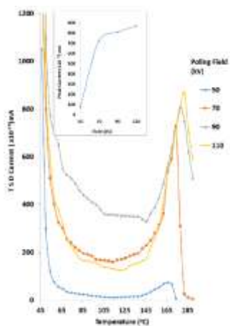
Figure 4 : TSDC thermograms for 90:10 polyblend samples poled at 70 oC with different poling fields (i.e. 50, 70, 90 and 110 kV/cm).
