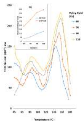
Figure 1 : TSDC thermogram for PMMA samples poled at 70 oC with different poling fields (i.e. 50, 70, 90 and 110 kV/cm).
